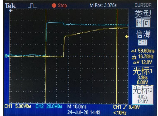
Output response &amp; load (12V / 0.5A)
