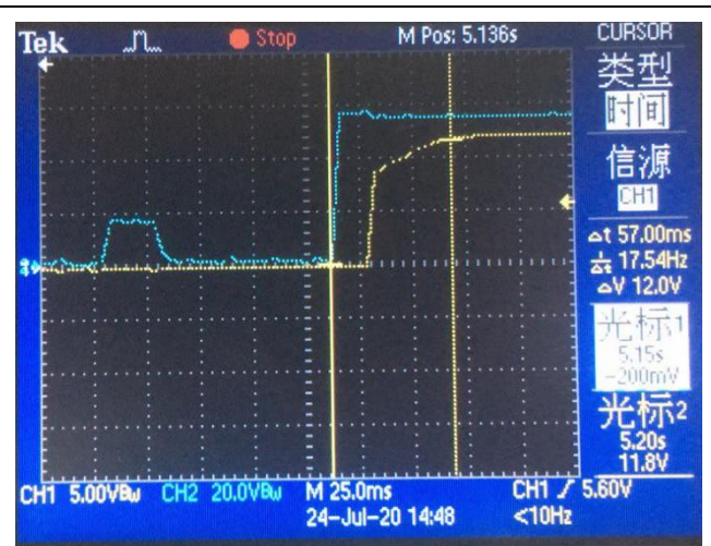
Output response &amp; load (12V / 1.1A)
