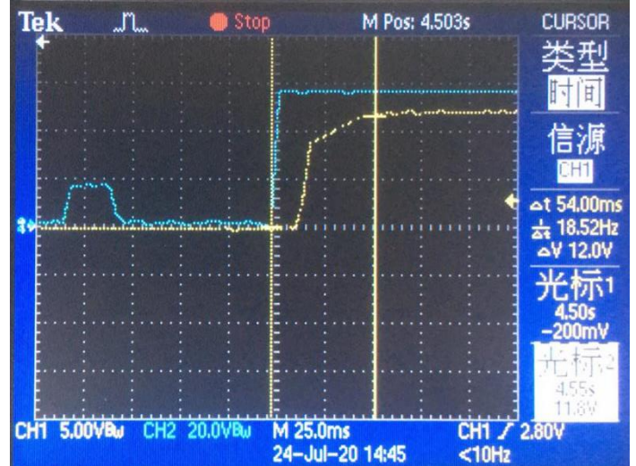
Output response &amp; load (12V / 0.01A)
